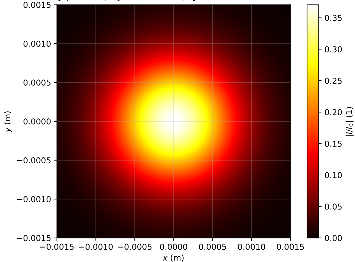
Intensity profile I(x, y, z = 3.025m)/I_0 , P_{in}=0.2P_{cr} , artificial time
